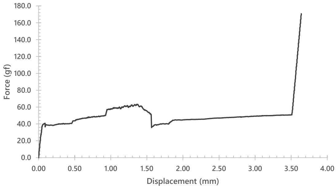
Kailh Mix-5 Blue (Upstroke)
